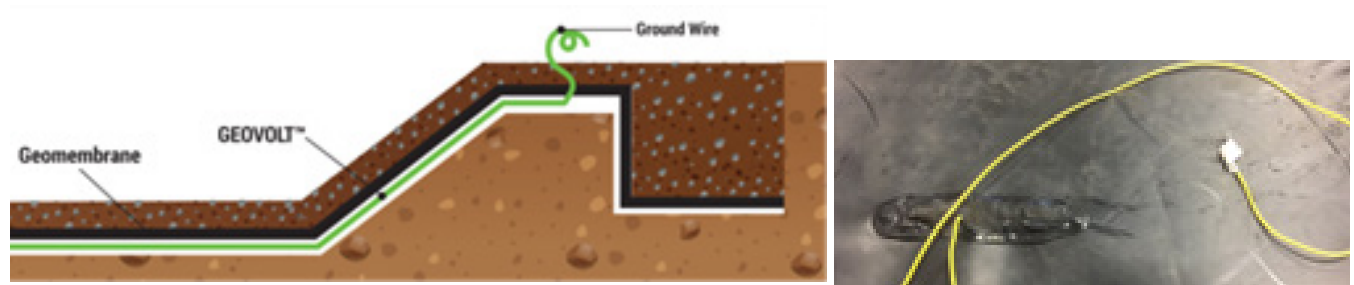
Figure 8. Exposed ground wire for future dipole testing using Geovolt
