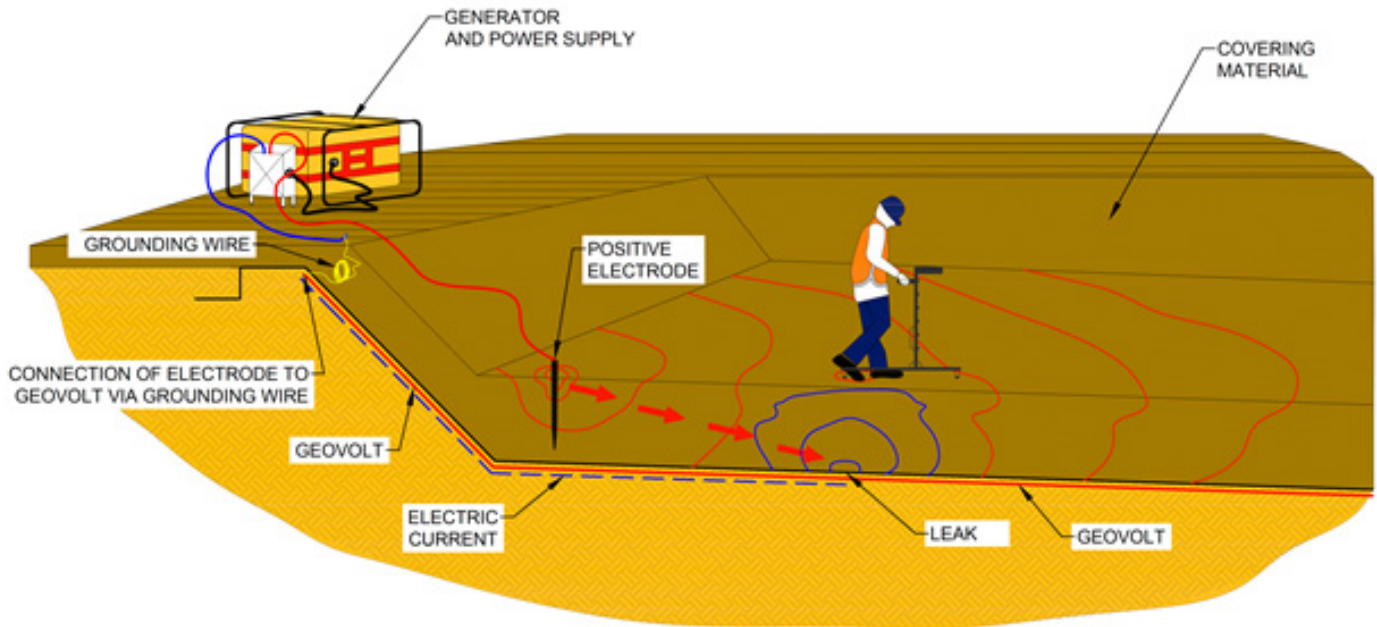
Figure 1. Schematic showing ELL performed using Geovolt in a covered application
