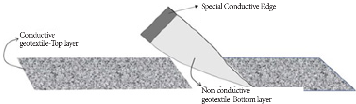
Figure 2. Schematic showing an overlap
